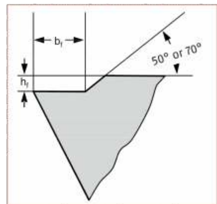
Fig. 20: Cross-section through a chip breaking element ground into the tool
