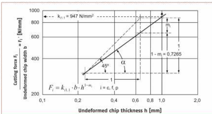
Fig. 13: Graphical determination of the parameters k_{cl,1} and (1-m_c) with i = c, f or p [8]
